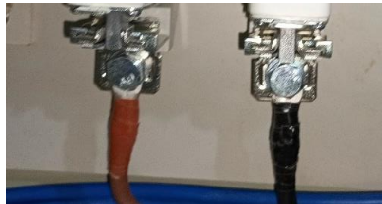
✓ 線耳應以絕緣膠帶包裹
