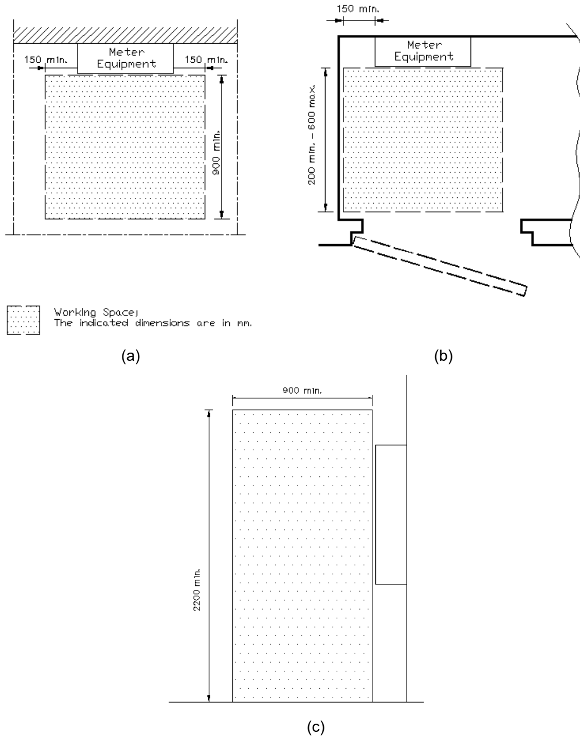
Figure 10.1 – Meter installed (a) in general region; (b) in electrical duct; (c) Working space in side view
