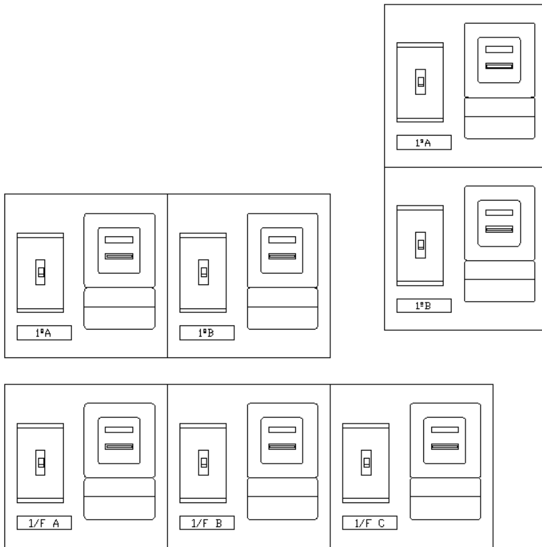
Figure 10.2 – Typical Meter Panel Arrangement
