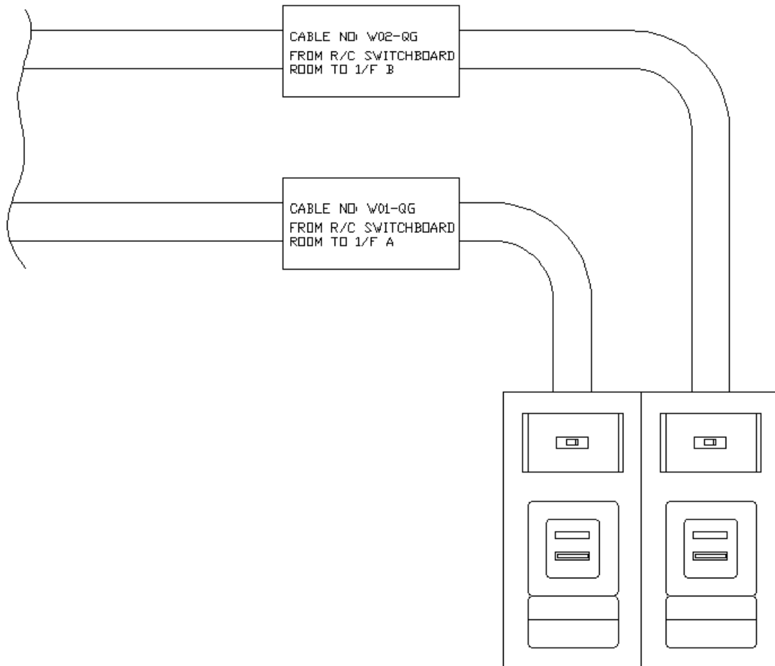
Figure 10.3 – Typical Cable Label
